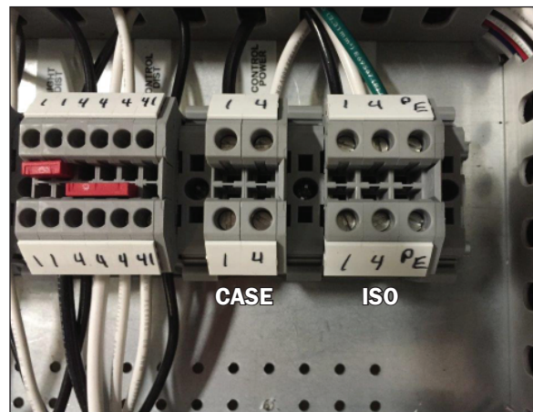
Fig. 8 Field wire connections
