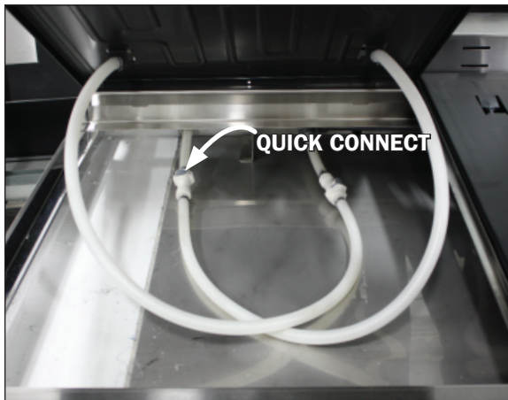
Fig. 19 Quick connect engaged
