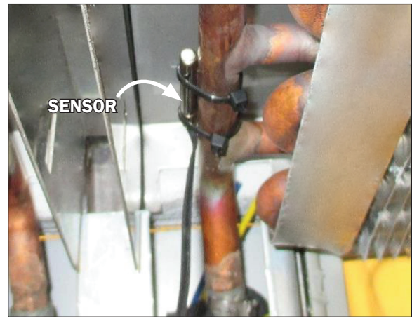
Fig. 4 Gravity coil sensor
